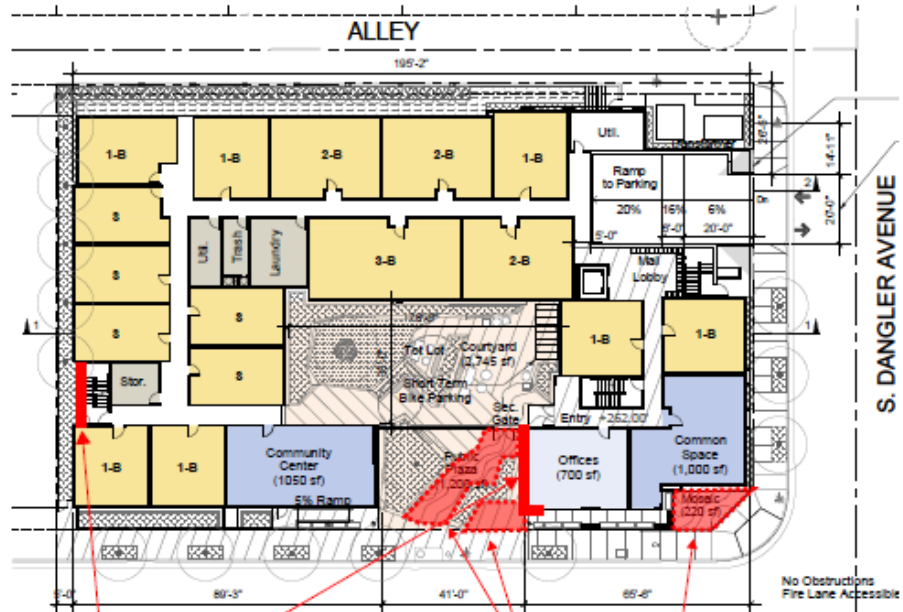
GROUND LEVEL PLAN
